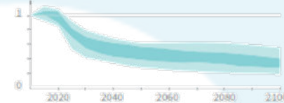
Black carbon emissions
