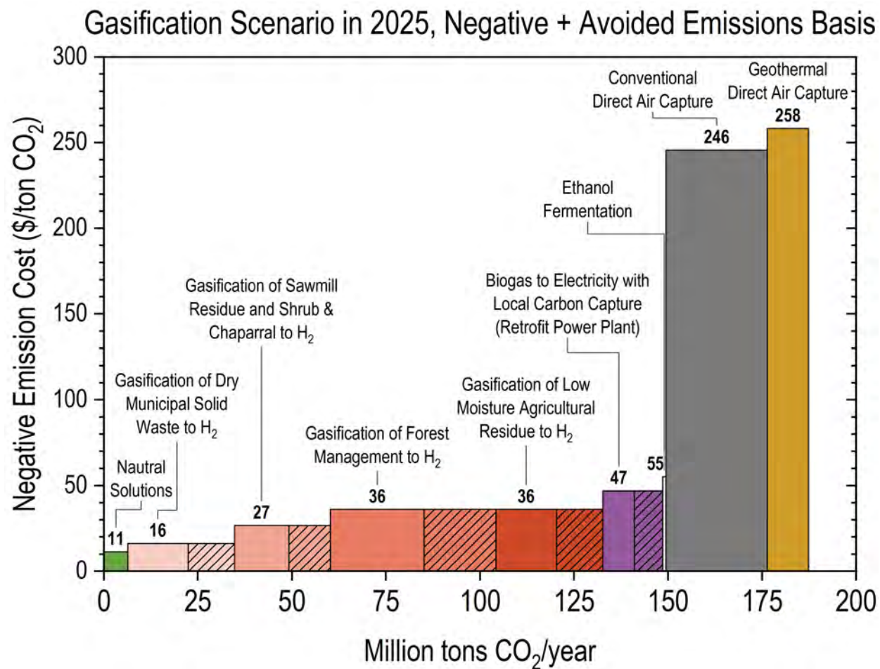
Figure S5 - Total cost curve for gasification scenario, 2025, negative and avoided emissions basis. Hatched areas represent avoided emissions. The total (integrated) system cost for this scenario is 14.1 billion $ per year.
