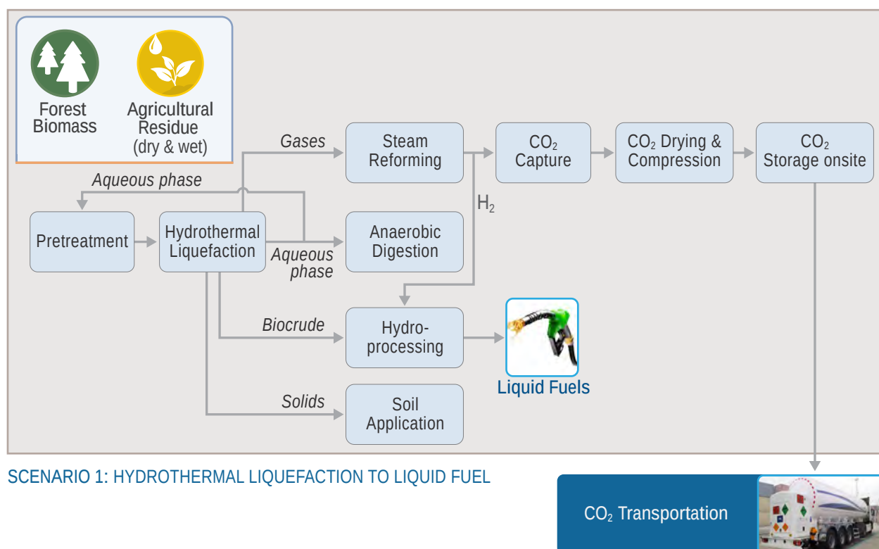
Figure 24. Simplified block flow diagram and system boundary of hydrothermal liquefaction to liquid fuel with carbon capture.
