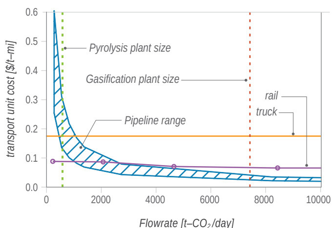
Figure 57. Unit cost to transport \text{CO}_2 by three modes over 150 mi. Vertical dashed lines mark the calculated \text{CO}_2 capture rates at typical pyrolysis and gasification plants.
